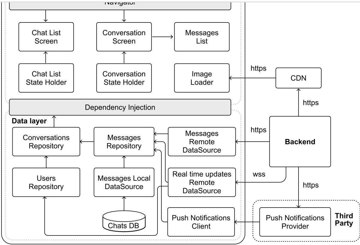
Figure 9: High-level mobile architecture of our chat system
